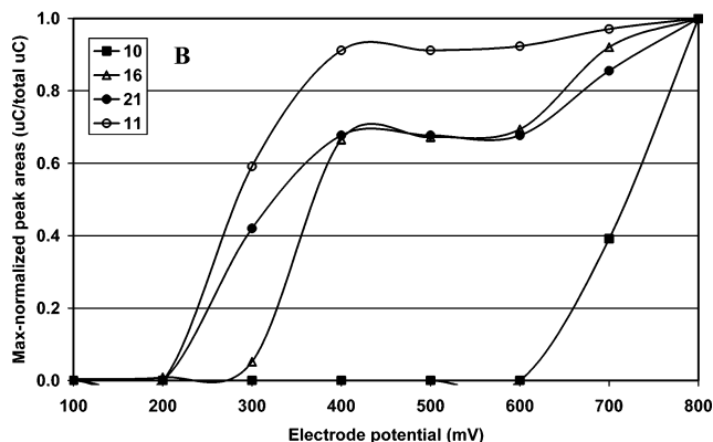
Figure 6. HDVs of partly identified or nonidentified compounds in strawberry fruits: (A) peak 39 (■); peak 5 (△); peak 27 (●); peak 38 (○); (B) peak 10 (■); peak 16 (△); peak 21 (●); peak 11 (○). Peak numbers refer to Tables 1 and 2.
